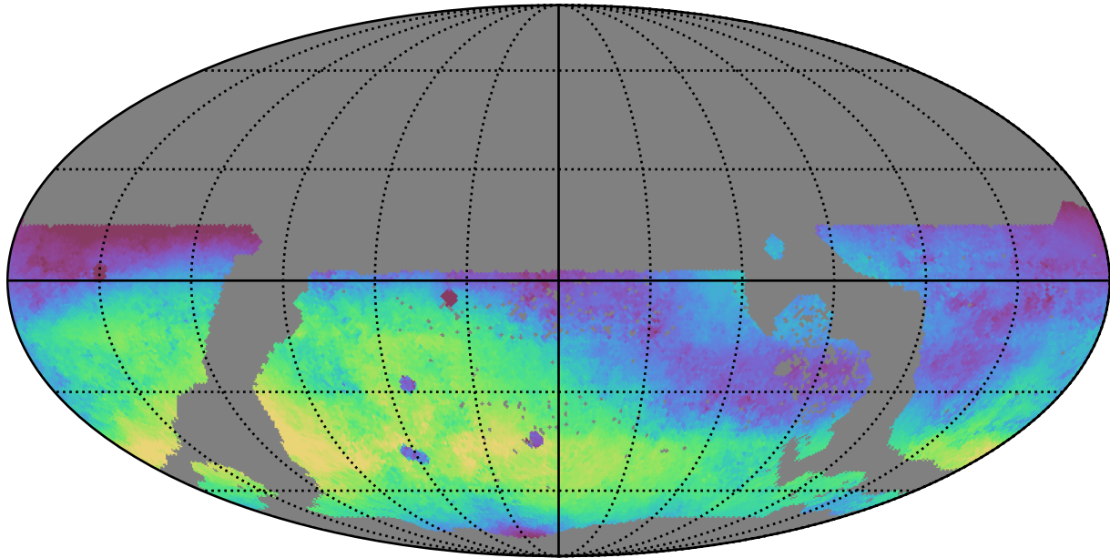
weather_cloudso0v3.4_10yrs WFD r band: Median skyBrightness
