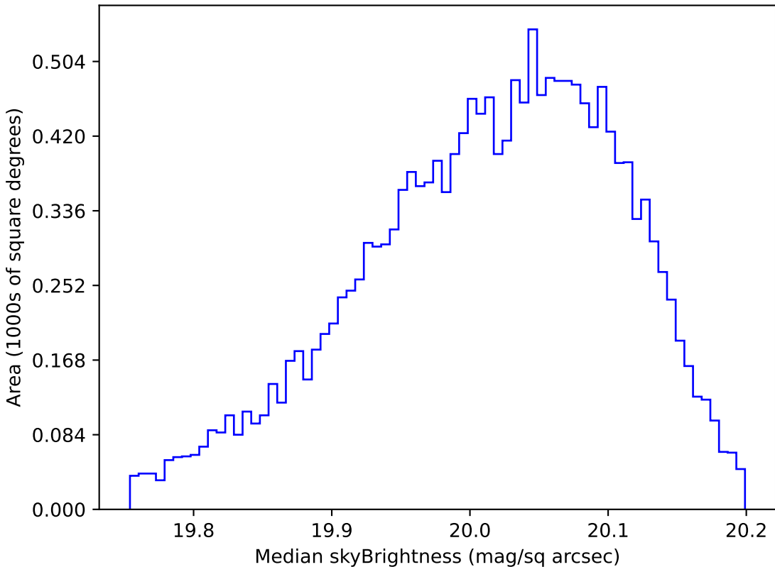
weather_cloudso0v3.4_10yrs WFD i band: Median skyBrightness
