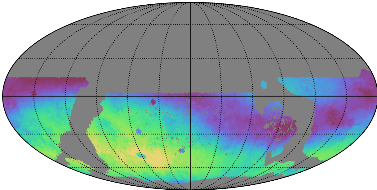
weather_cloudso0v3.4_10yrs WFD g band: Median skyBrightness
