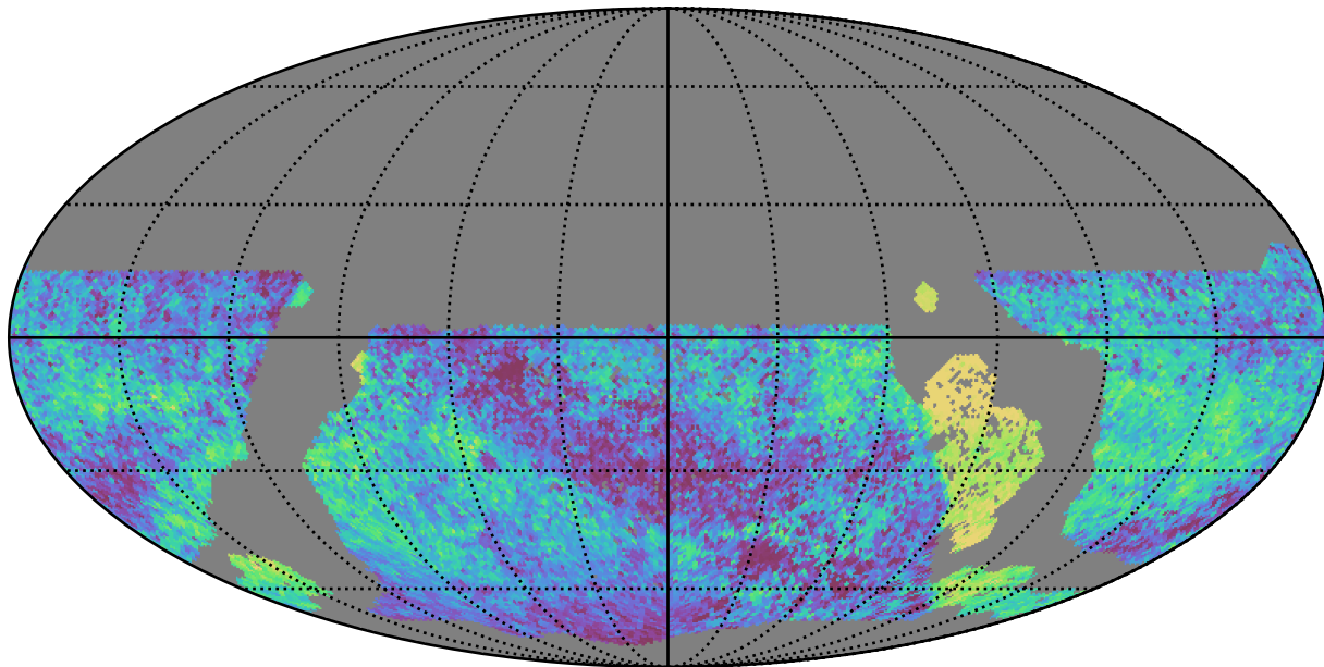
weather_cloudso0v3.4_10yrs WFD all bands: Median skyBrightness
