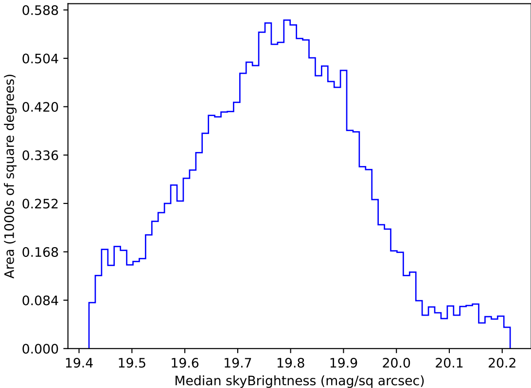
weather_cloudso0v3.4_10yrs WFD all bands: Median skyBrightness
