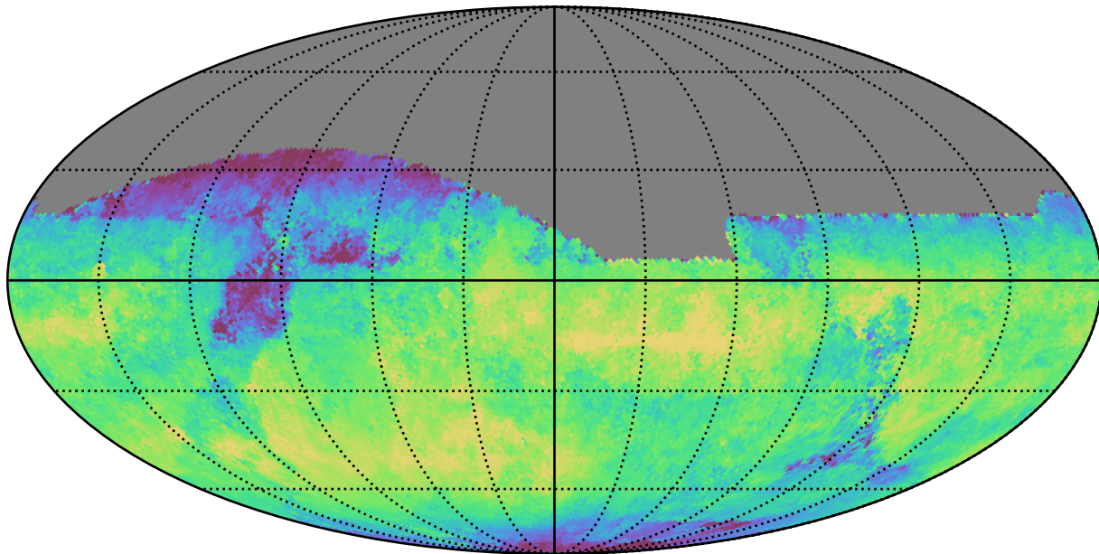
weather_cloudso0v3.4_10yrs All sky z band: Median skyBrightness
