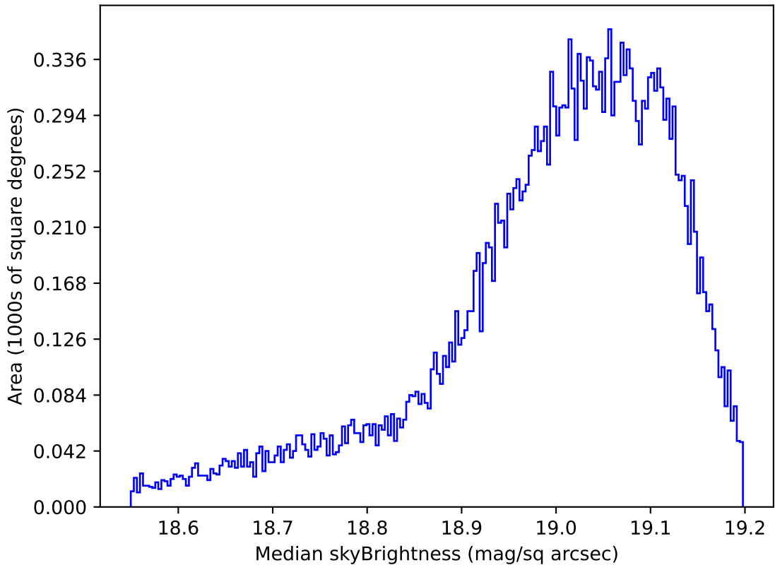
weather_cloudso0v3.4_10yrs All sky z band: Median skyBrightness
