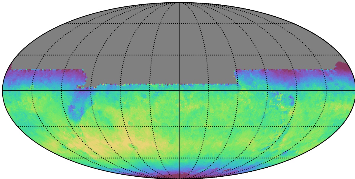
weather_cloudso0v3.4_10yrs All sky y band: Median skyBrightness
