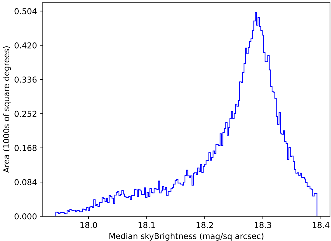
weather_cloudso0v3.4_10yrs All sky y band: Median skyBrightness
