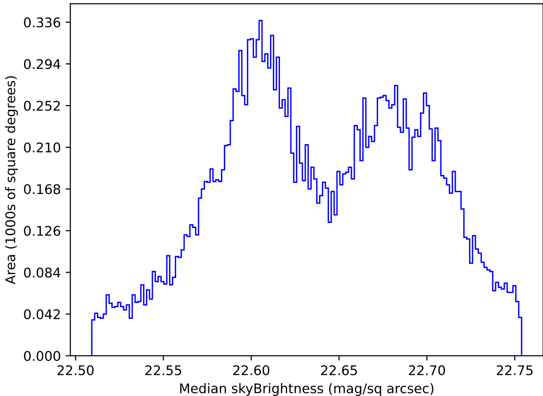
weather_cloudso0v3.4_10yrs All sky u band: Median skyBrightness
