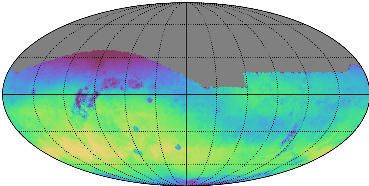
weather_cloudso0v3.4_10yrs All sky r band: Median skyBrightness
