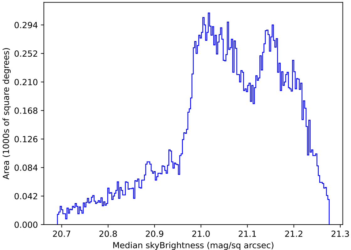
weather_cloudso0v3.4_10yrs All sky r band: Median skyBrightness
