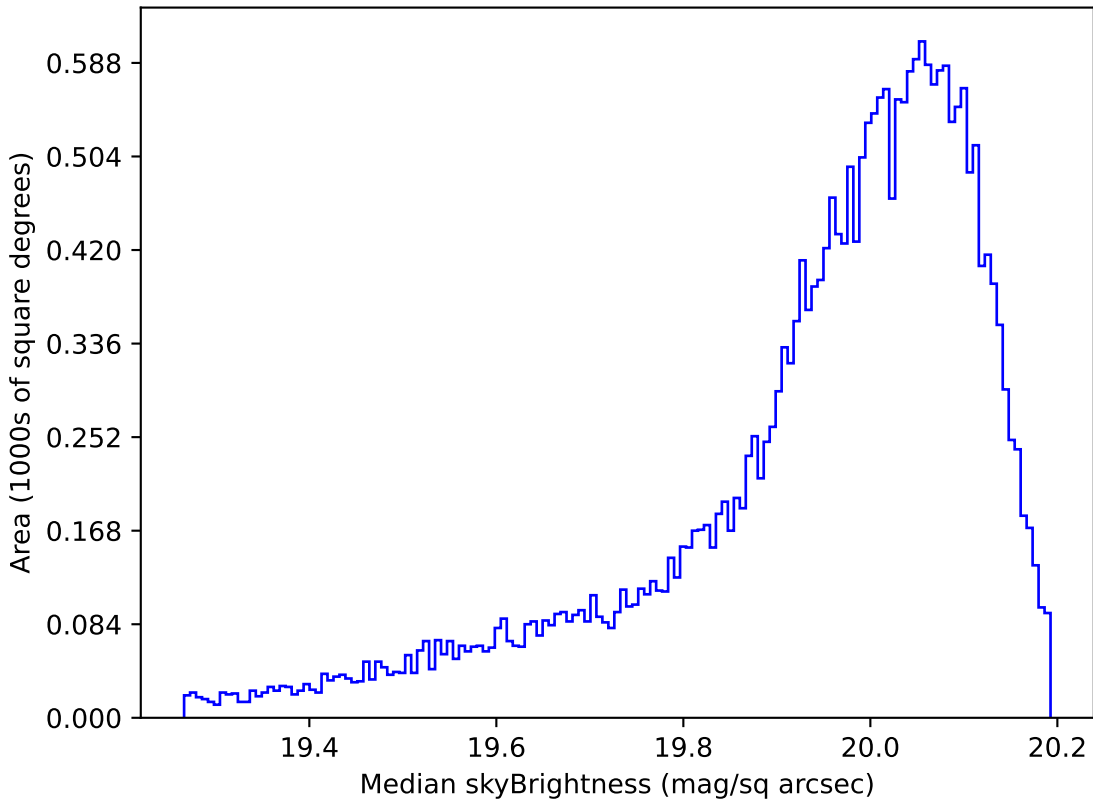
weather_cloudso0v3.4_10yrs All sky i band: Median skyBrightness
