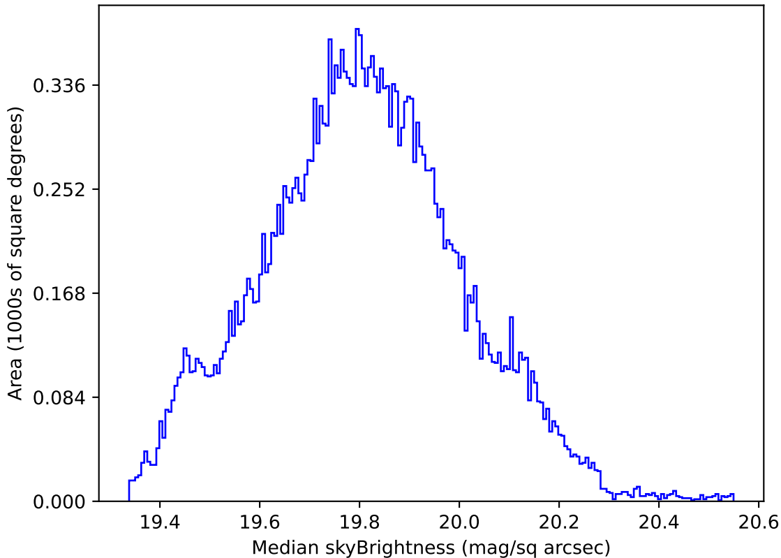
weather_cloudso0v3.4_10yrs All sky all bands: Median skyBrightness
