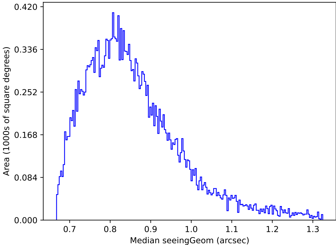
weather_cloudso0v3.4_10yrs Yr 1 z band: Median seeingGeom
