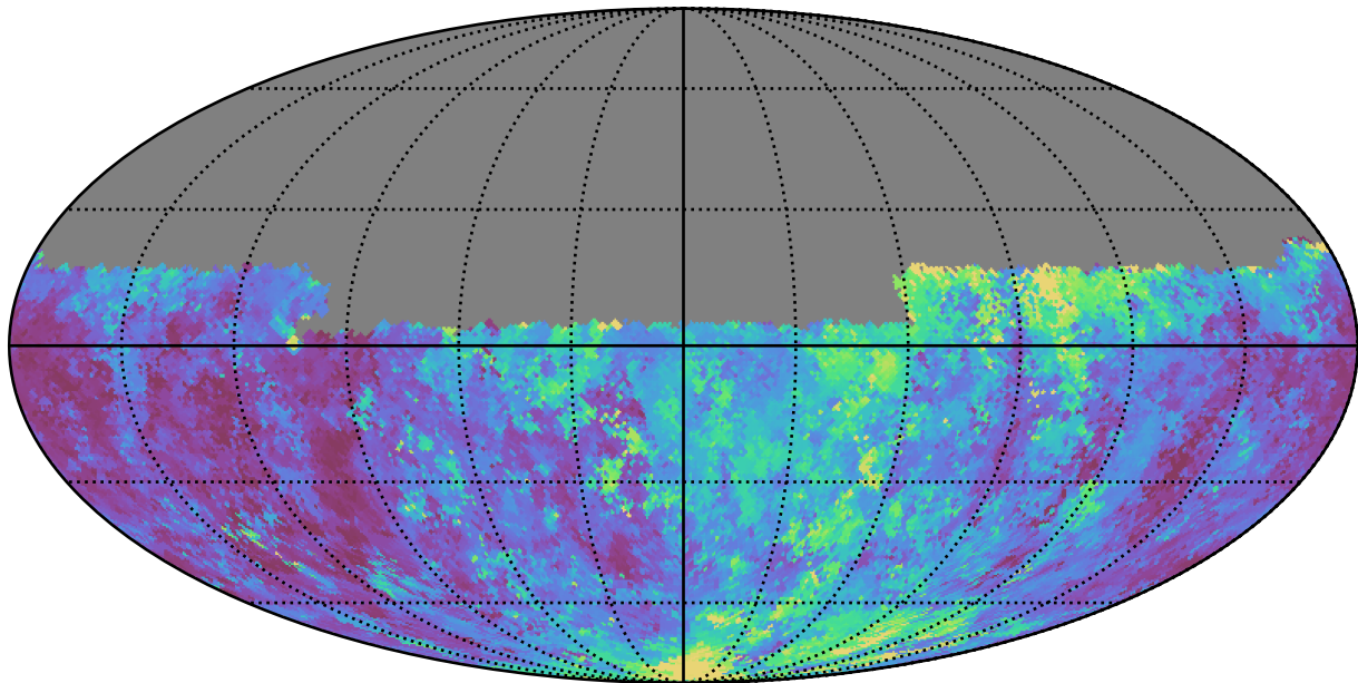
weather_cloudso0v3.4_10yrs Yr 1 u band: Median seeingGeom
