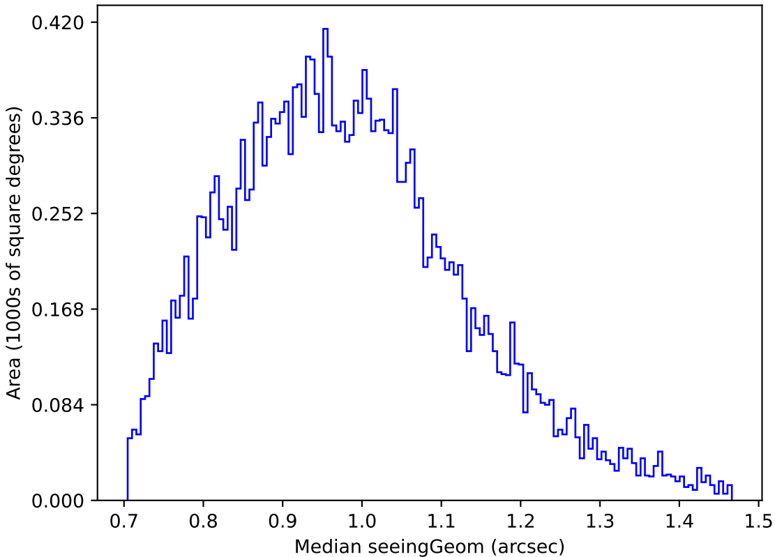
weather_cloudso0v3.4_10yrs Yr 1 u band: Median seeingGeom
