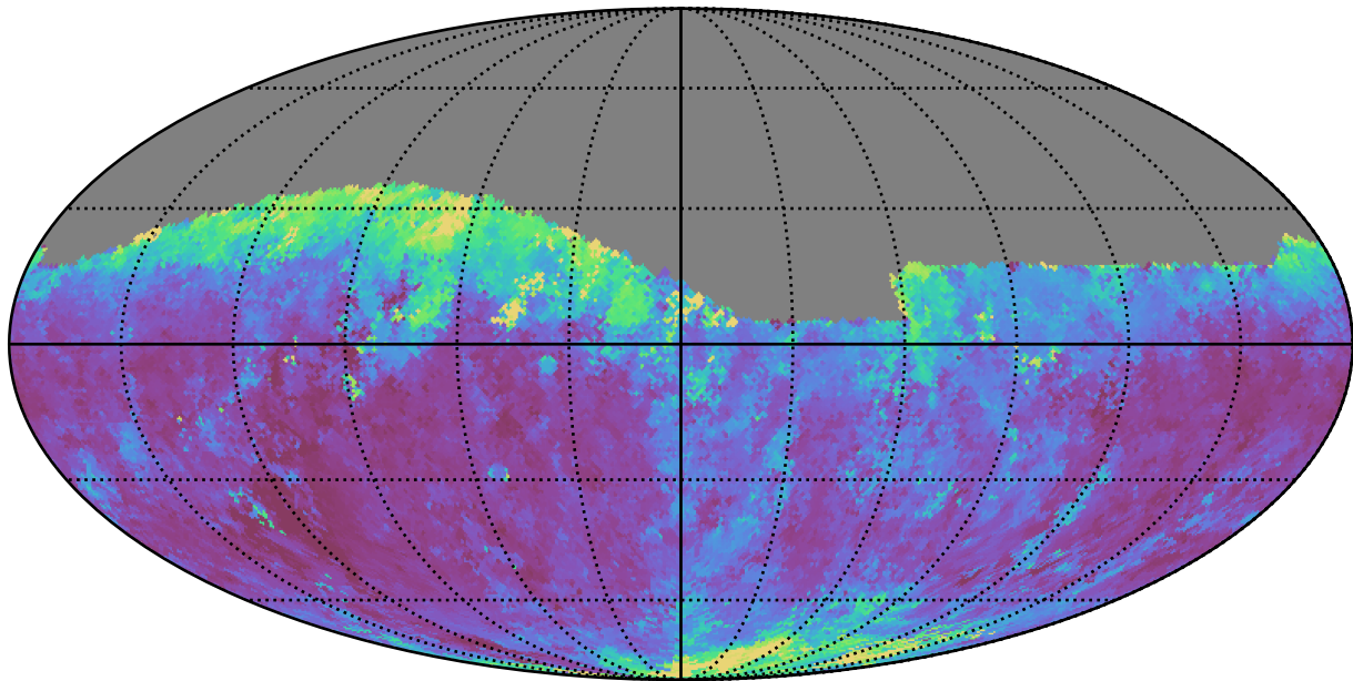
weather_cloudso0v3.4_10yrs Yr 1 r band: Median seeingGeom
