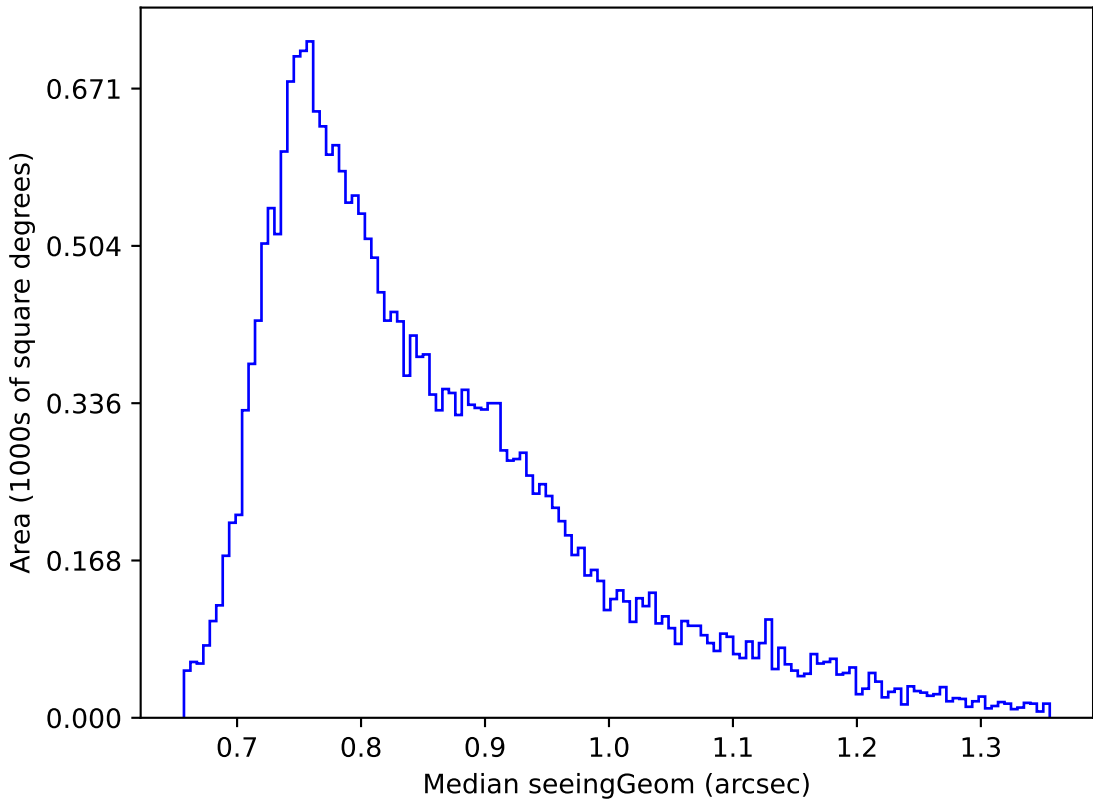
weather_cloudso0v3.4_10yrs Yr 1 r band: Median seeingGeom
