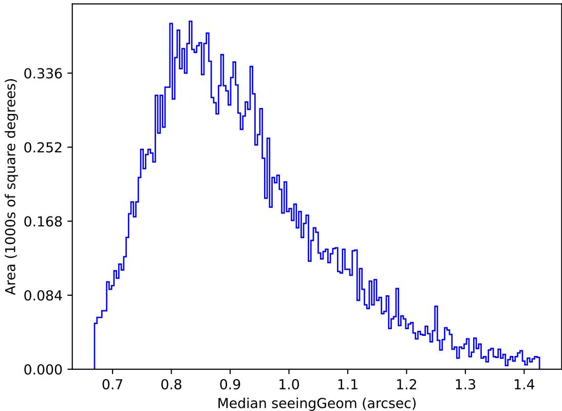
weather_cloudso0v3.4_10yrs Yr 1 g band: Median seeingGeom
