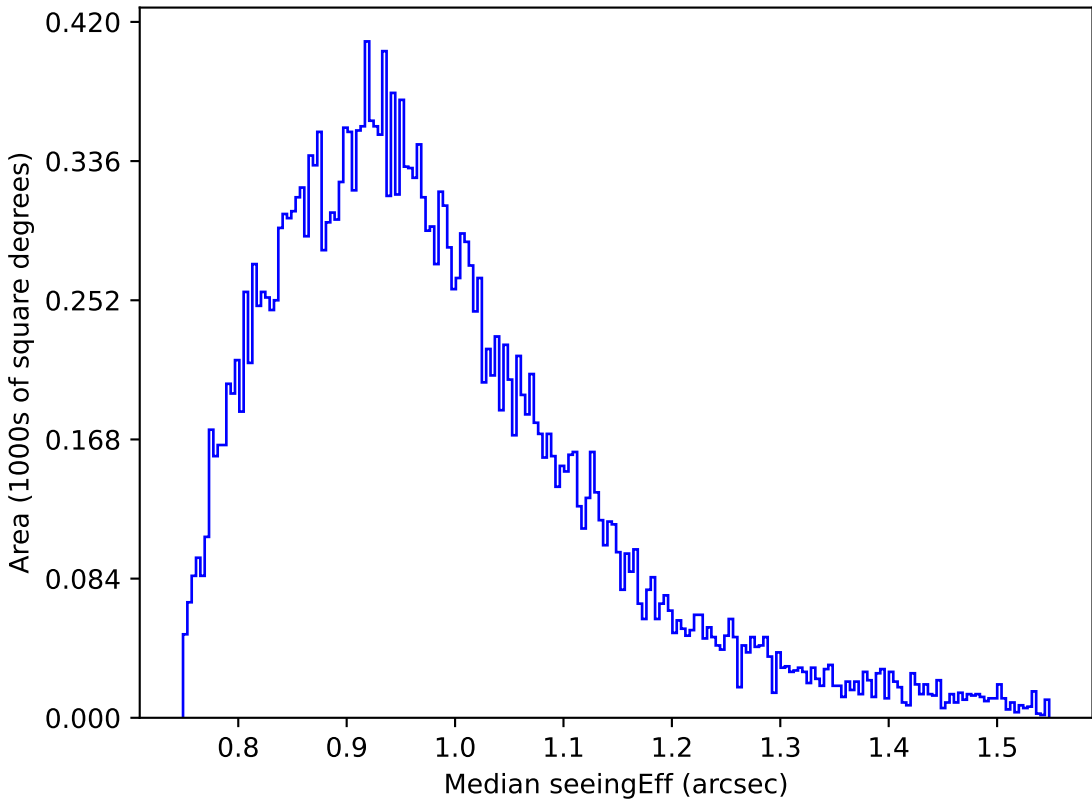
weather_cloudso0v3.4_10yrs Yr 1 z band: Median seeingEff
