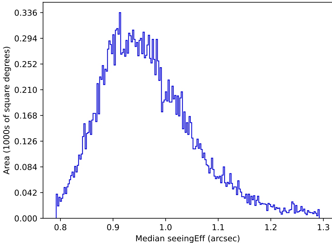
weather_cloudso0v3.4_10yrs Yr 1 y band: Median seeingEff
