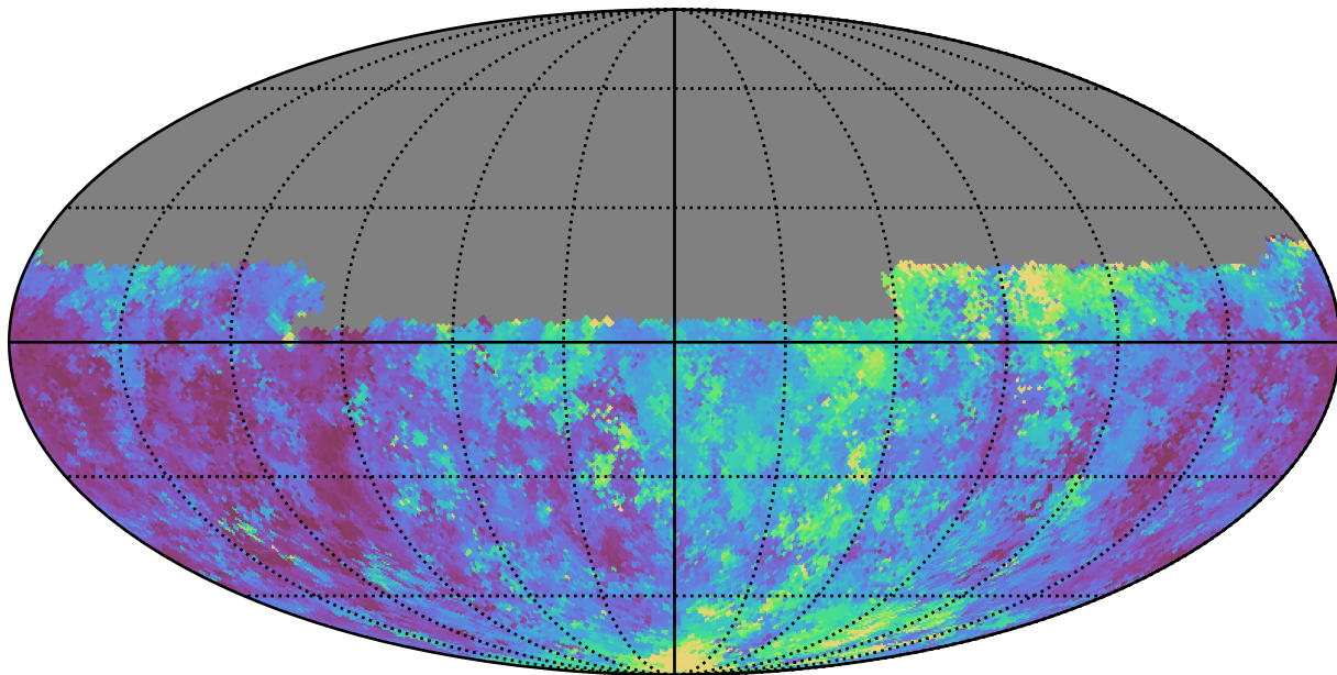
weather_cloudso0v3.4_10yrs Yr 1 u band: Median seeingEff
