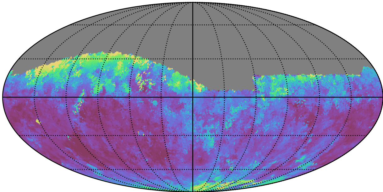
weather_cloudso0v3.4_10yrs Yr 1 i band: Median seeingEff
