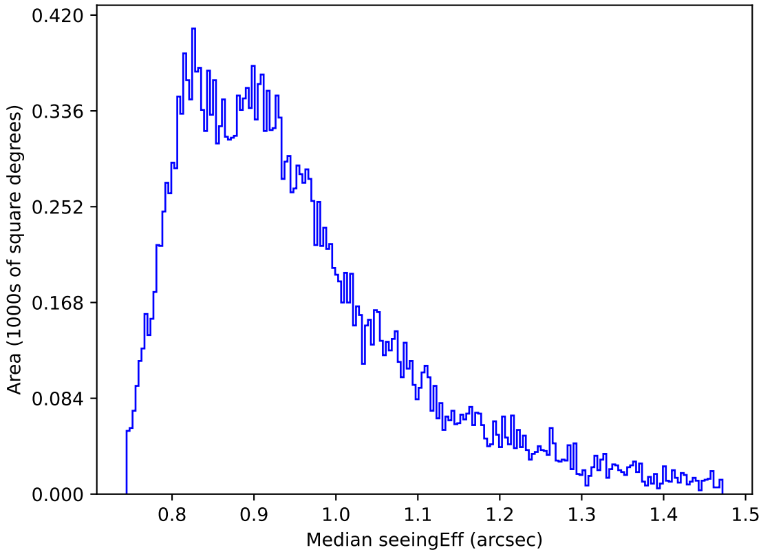
weather_cloudso0v3.4_10yrs Yr 1 i band: Median seeingEff
