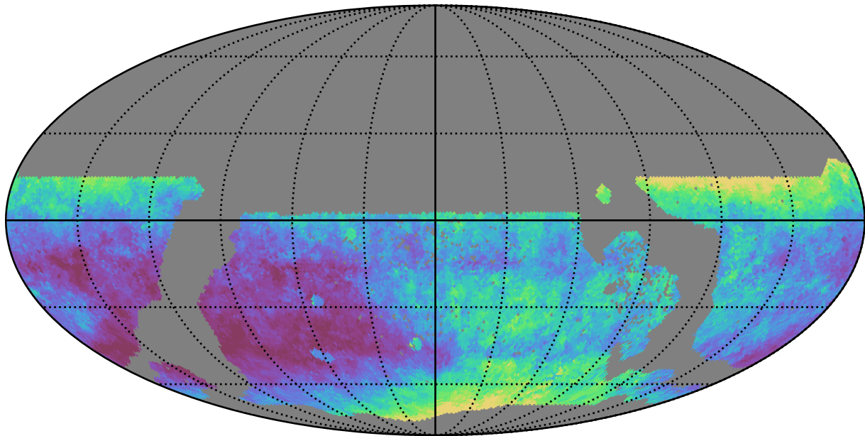
weather_cloudso0v3.4_10yrs WFD z band: Median seeingEff
