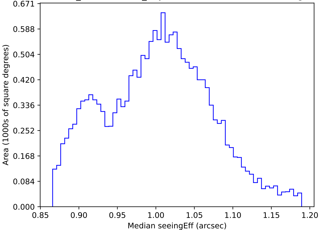
weather_cloudso0v3.4_10yrs WFD z band: Median seeingEff
