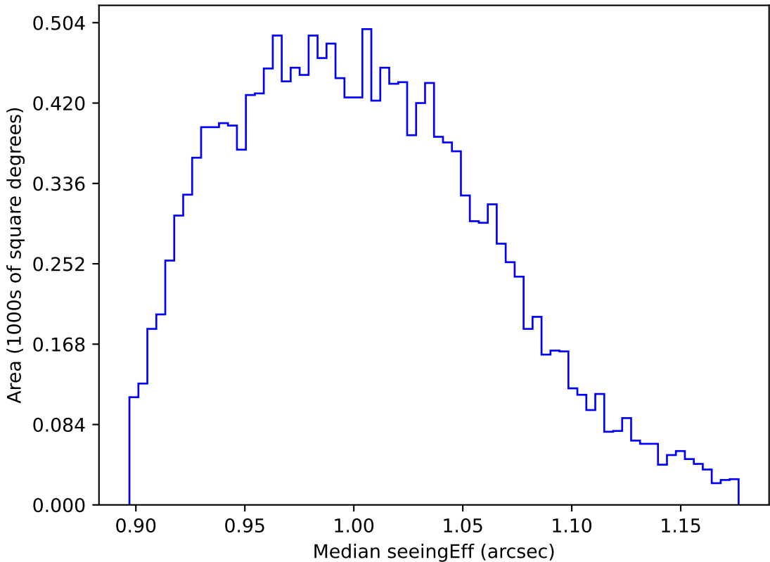
weather_cloudso0v3.4_10yrs WFD y band: Median seeingEff
