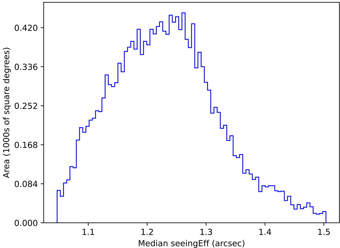
weather_cloudso0v3.4_10yrs WFD u band: Median seeingEff
