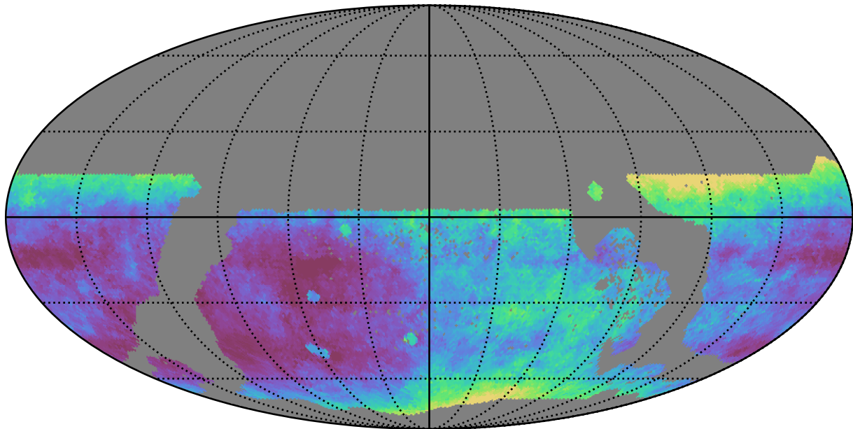
weather_cloudso0v3.4_10yrs WFD r band: Median seeingEff
