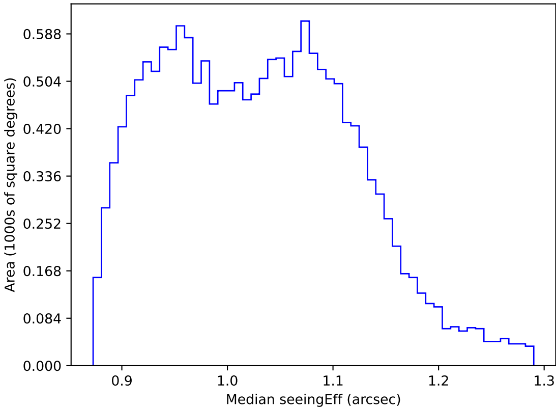
weather_cloudso0v3.4_10yrs WFD r band: Median seeingEff
