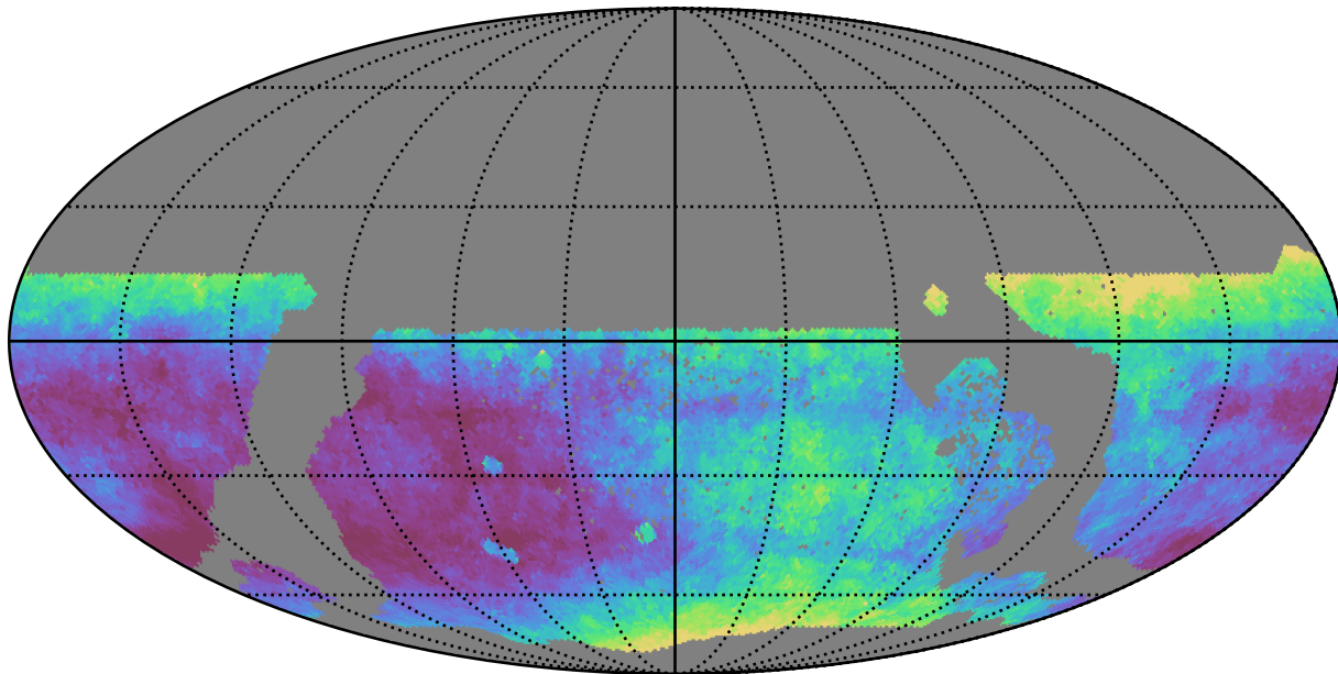
weather_cloudso0v3.4_10yrs WFD i band: Median seeingEff
