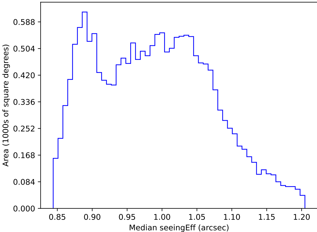
weather_cloudso0v3.4_10yrs WFD i band: Median seeingEff
