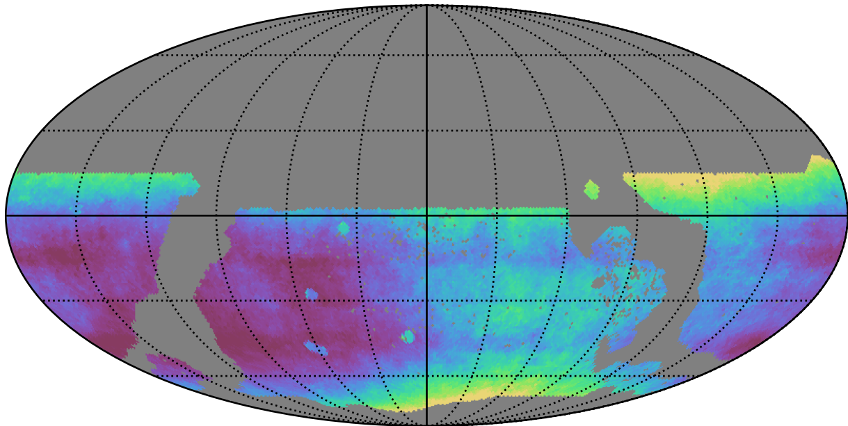
weather_cloudso0v3.4_10yrs WFD all bands: Median seeingEff
