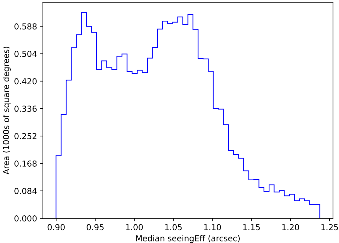
weather_cloudso0v3.4_10yrs WFD all bands: Median seeingEff
