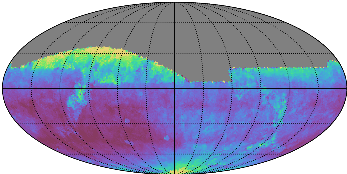
weather_cloudso0v3.4_10yrs All sky z band: Median seeingEff
