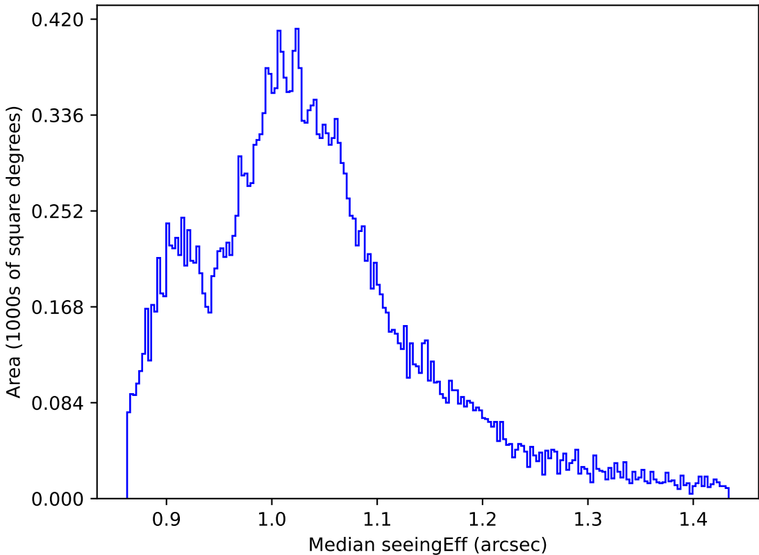
weather_cloudso0v3.4_10yrs All sky z band: Median seeingEff
