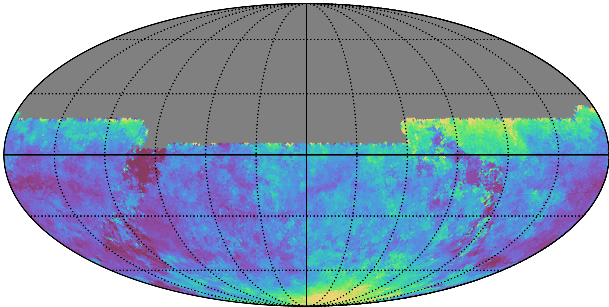
weather_cloudso0v3.4_10yrs All sky u band: Median seeingEff
