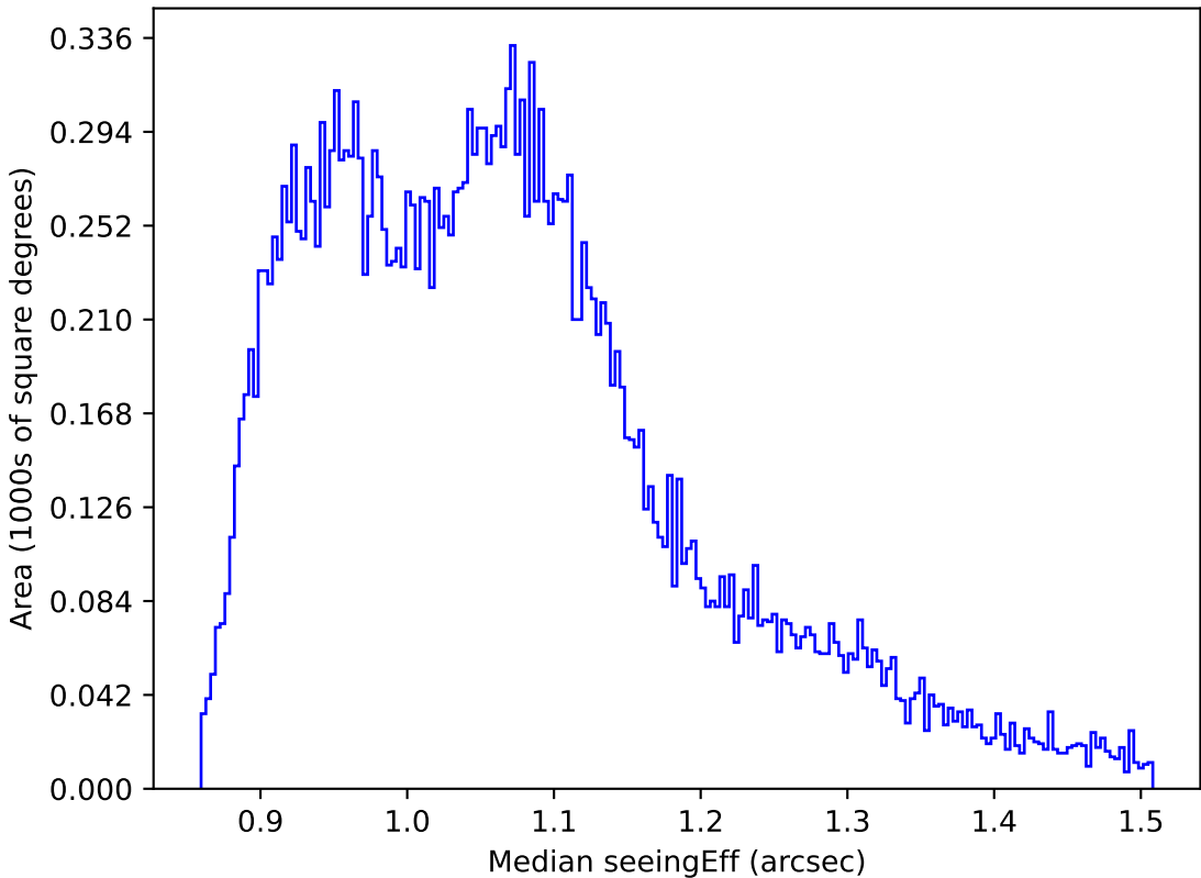
weather_cloudso0v3.4_10yrs All sky r band: Median seeingEff
