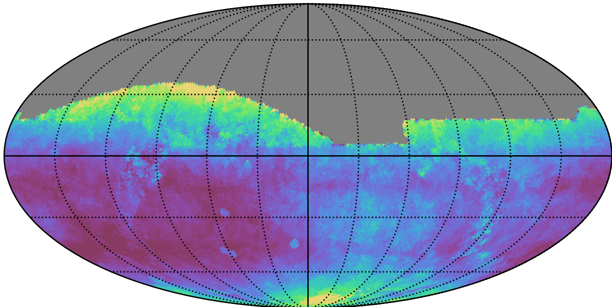
weather_cloudso0v3.4_10yrs All sky i band: Median seeingEff
