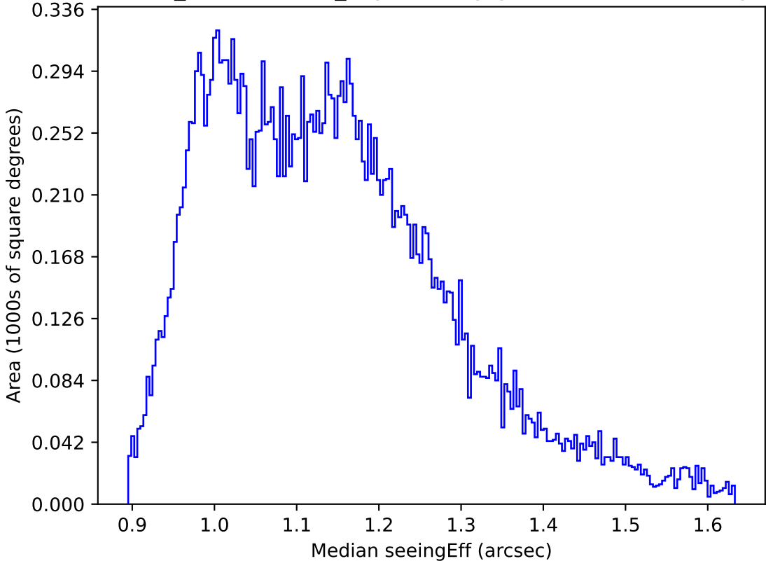
weather_cloudso0v3.4_10yrs All sky g band: Median seeingEff
