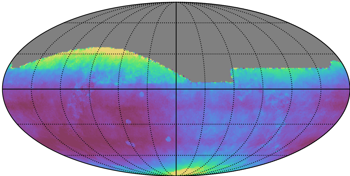
weather_cloudso0v3.4_10yrs All sky all bands: Median seeingEff
