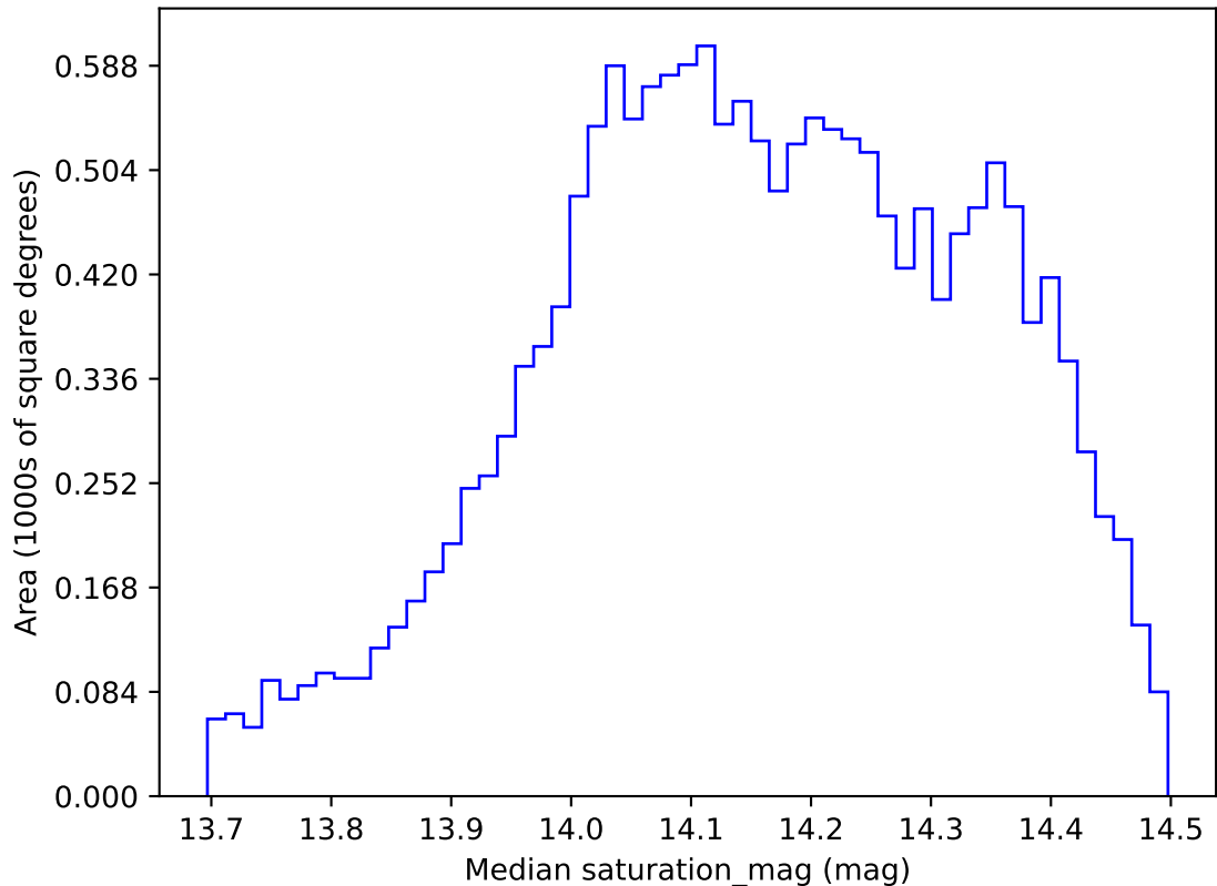
weather_cloudso0v3.4_10yrs WFD all bands: Median saturation_mag
