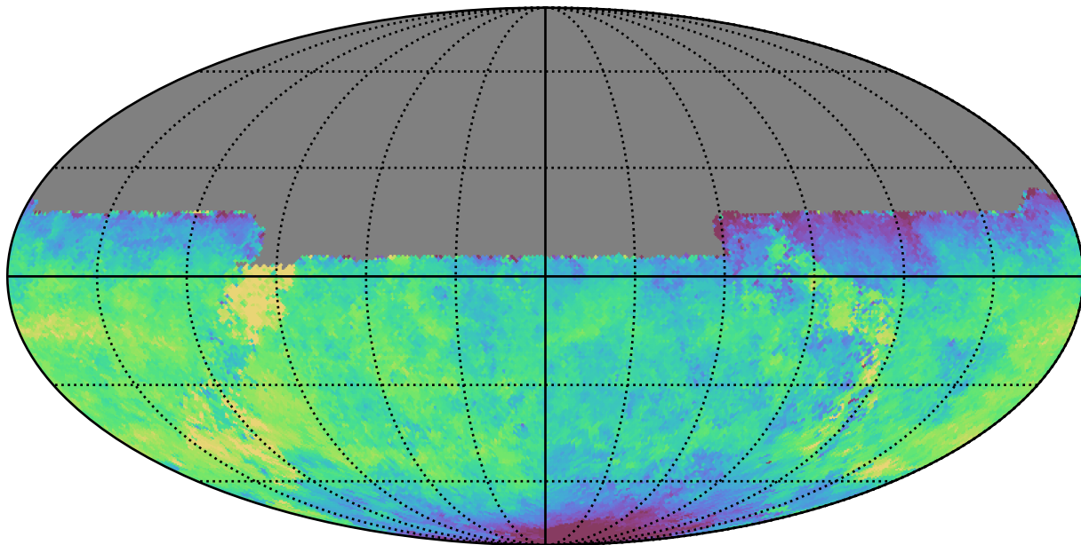
weather_cloudso0v3.4_10yrs All sky u band: Median saturation_mag
