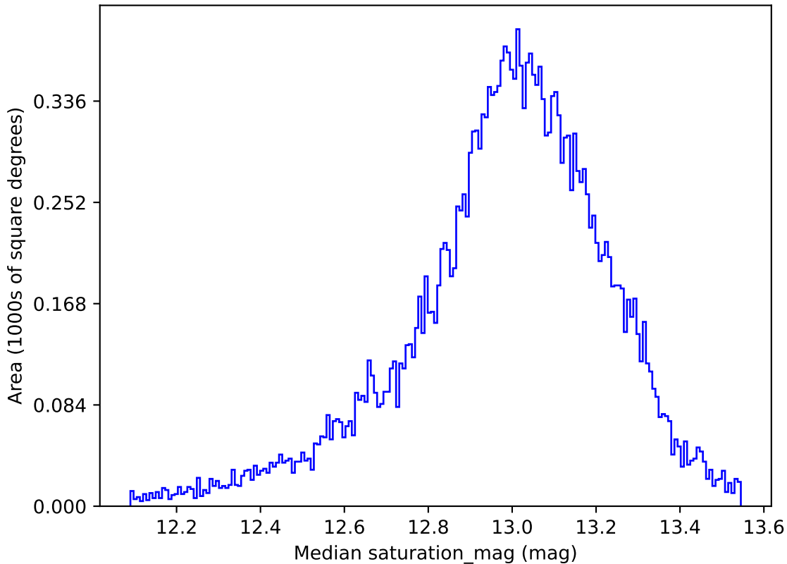
weather_cloudso0v3.4_10yrs All sky u band: Median saturation_mag
