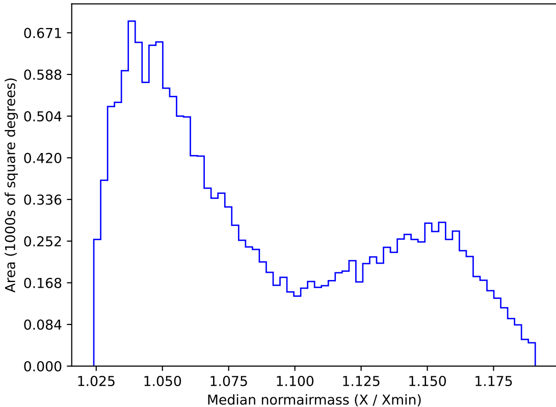
weather_cloudso0v3.4_10yrs WFD z band: Median normairmass
