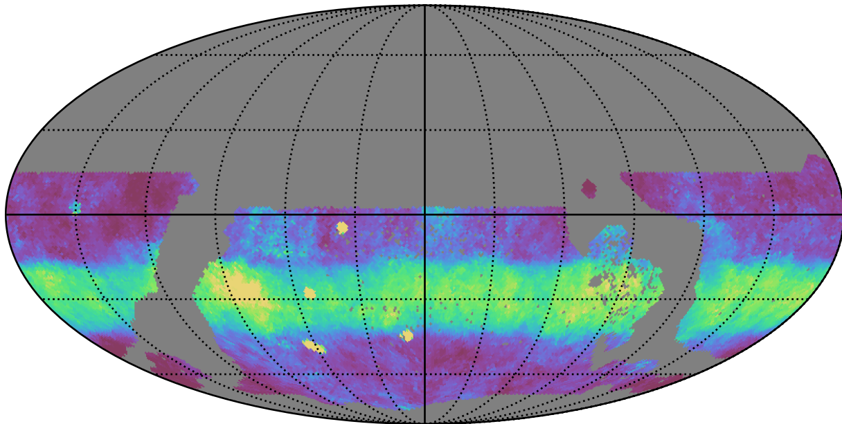
weather_cloudso0v3.4_10yrs WFD y band: Median normairmass
