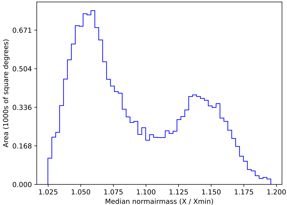
weather_cloudso0v3.4_10yrs WFD y band: Median normairmass
