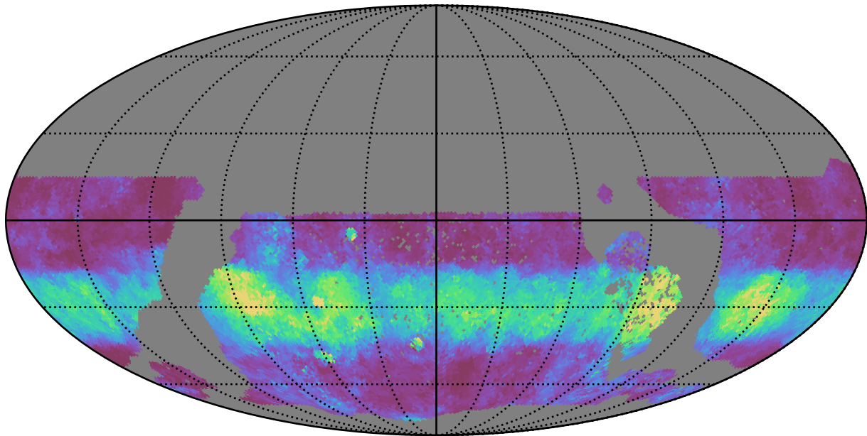
weather_cloudso0v3.4_10yrs WFD u band: Median normairmass
