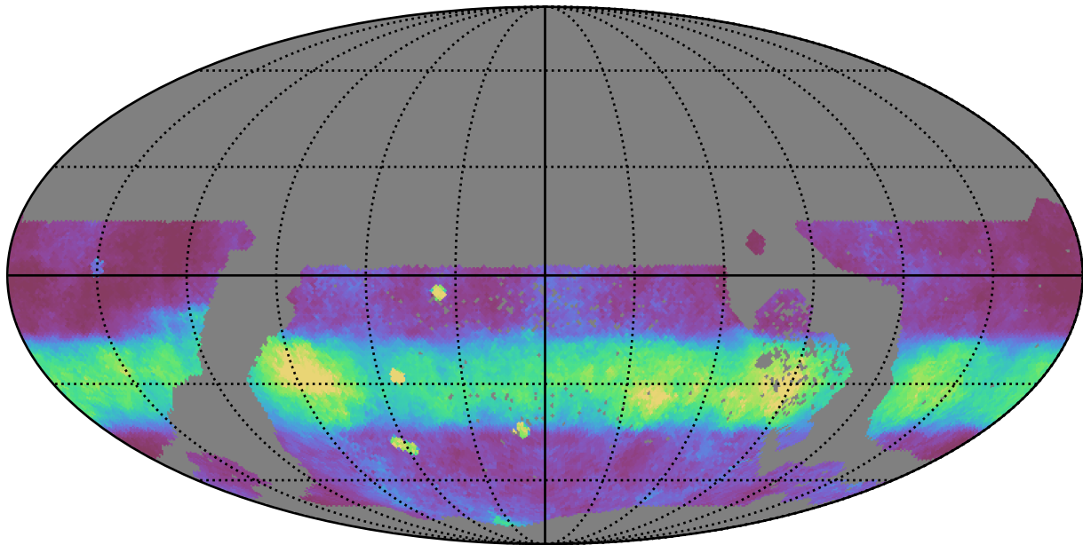
weather_cloudso0v3.4_10yrs WFD r band: Median normairmass
